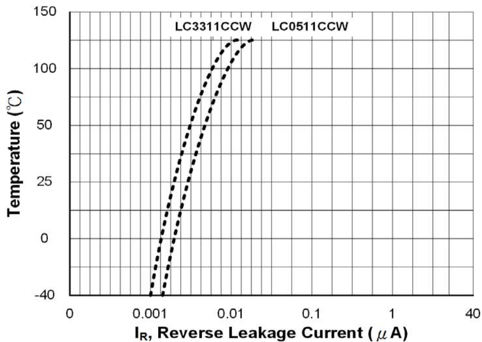
Figure 5. Typic Reverse Leakage vs. Temperature
