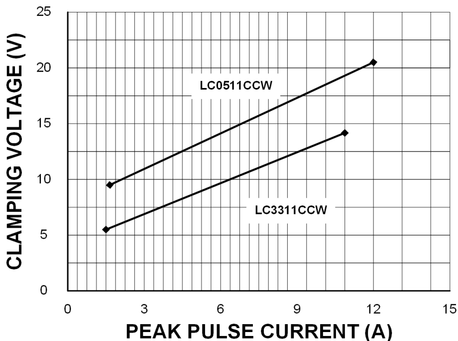
Figure 3. Clamping Voltage vs. Peak Pulse Current (tp=8/20us)
